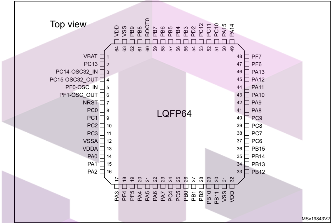
Figure 3. LQFP64 package pinout
