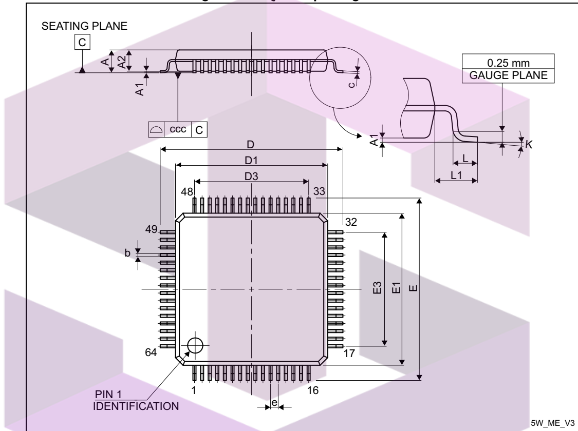
Figure 37. LQFP64 package outline
