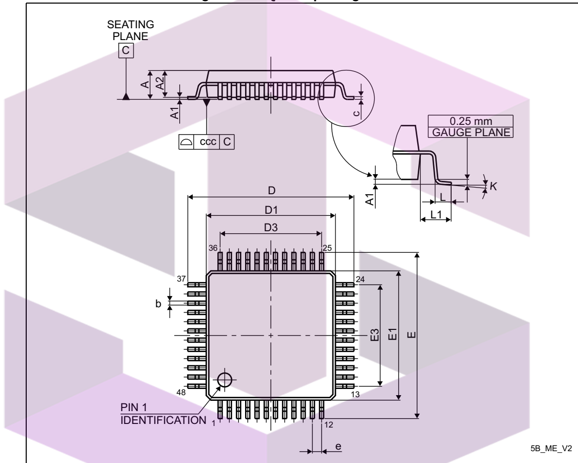
Figure 40. LQFP48 package outline
